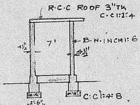
SECTION OF X-Y
