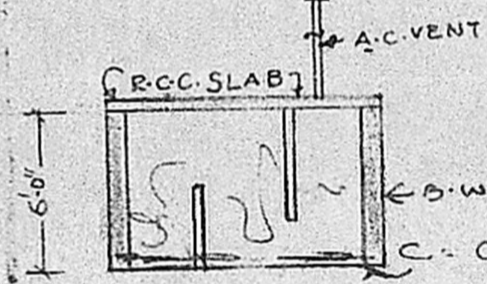
SECTION OF S-TANK
