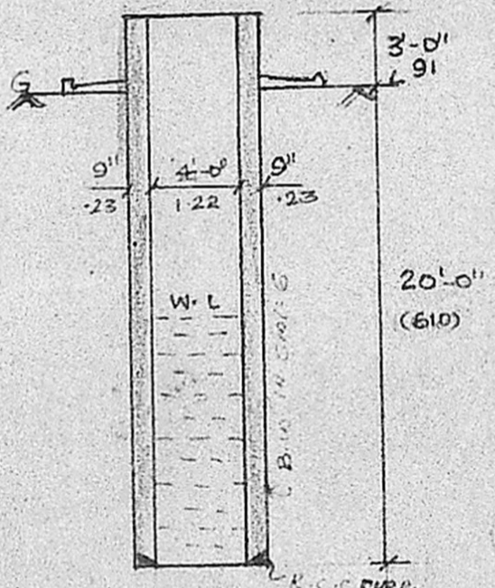
SECTION OF X-Y
