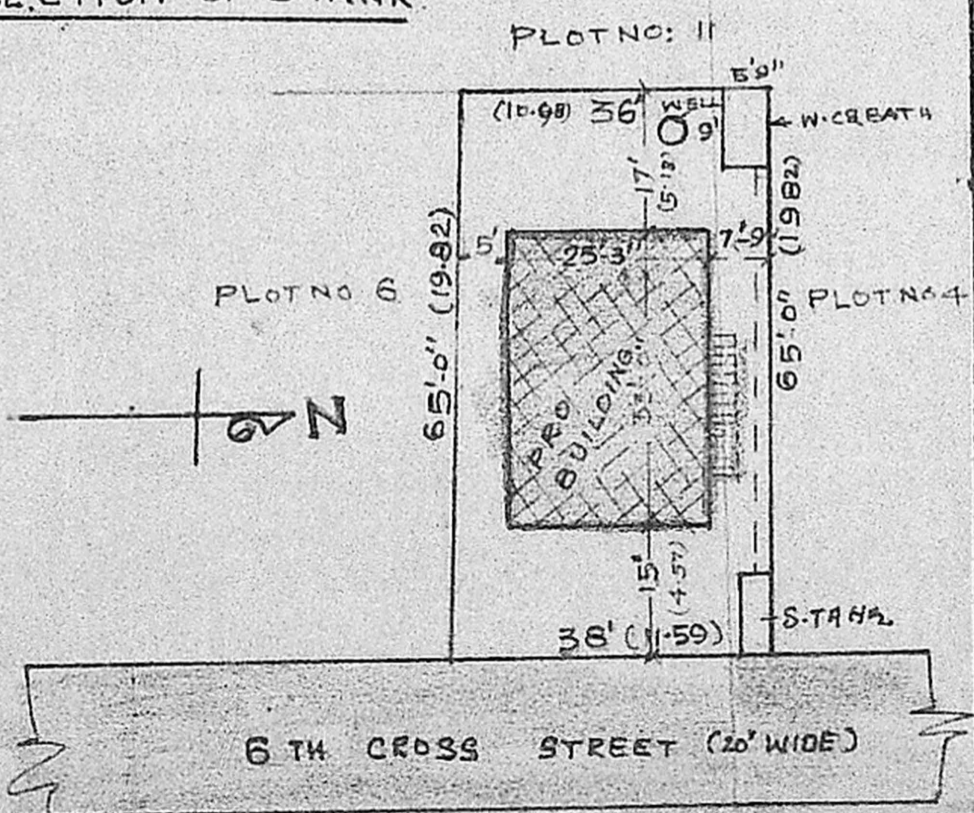
SCALE 1" = 24'-0" SITE PLAN
