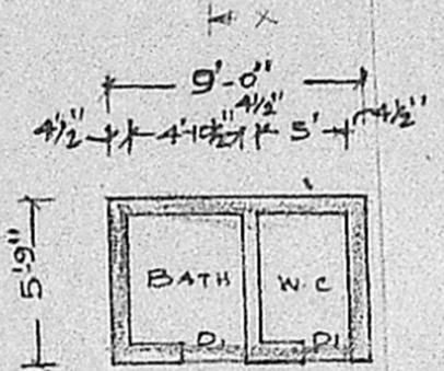
PLAN OF W.C. & BATH
